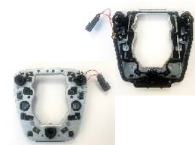
AIRBAG FRAME METAL FORMING / PLASTIC OVERMOULDING
