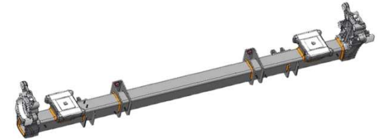
Rear Axle incl. welding and machining
